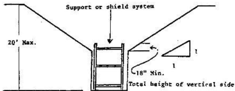
VERTICALLY SIDED LOWER PORTION
