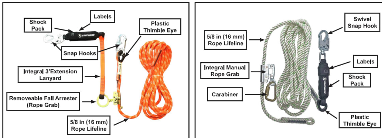
FIGURE 5 - COMPONENTS
