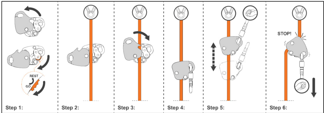
FIGURE 11 - SW-EX8000 INSTALLATION
