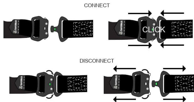
FIGURE 6 - BUCKLE OPERATION
