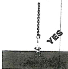
Photograph E. (Typical) Sling directly above and in line with the lifting shackle. (J and JA only)
