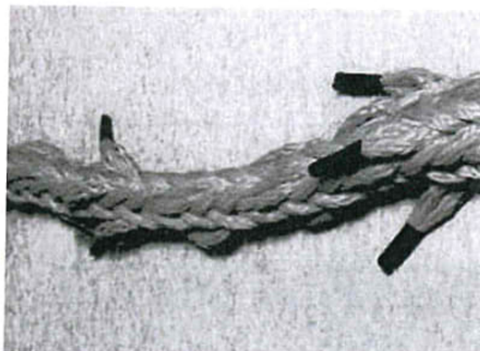
Figure 3: endless grommet sling with end-to-end splice
