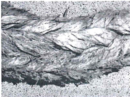
Excessive abrasion wear – volume of total rope in selected area is substantially reduced
